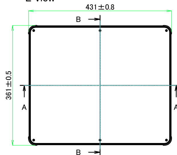
E view
